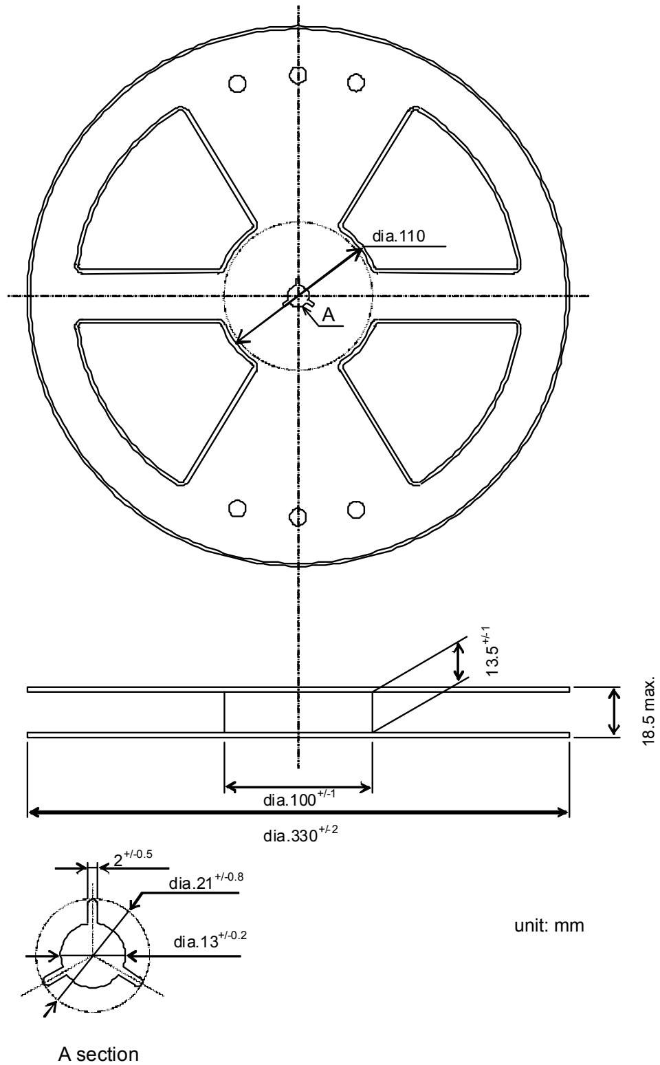
Fig.3. Reel specification
